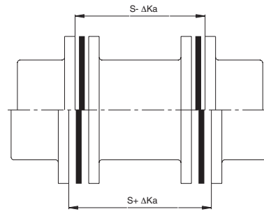
Axial misalignment
