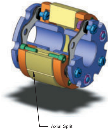
Axial Split
